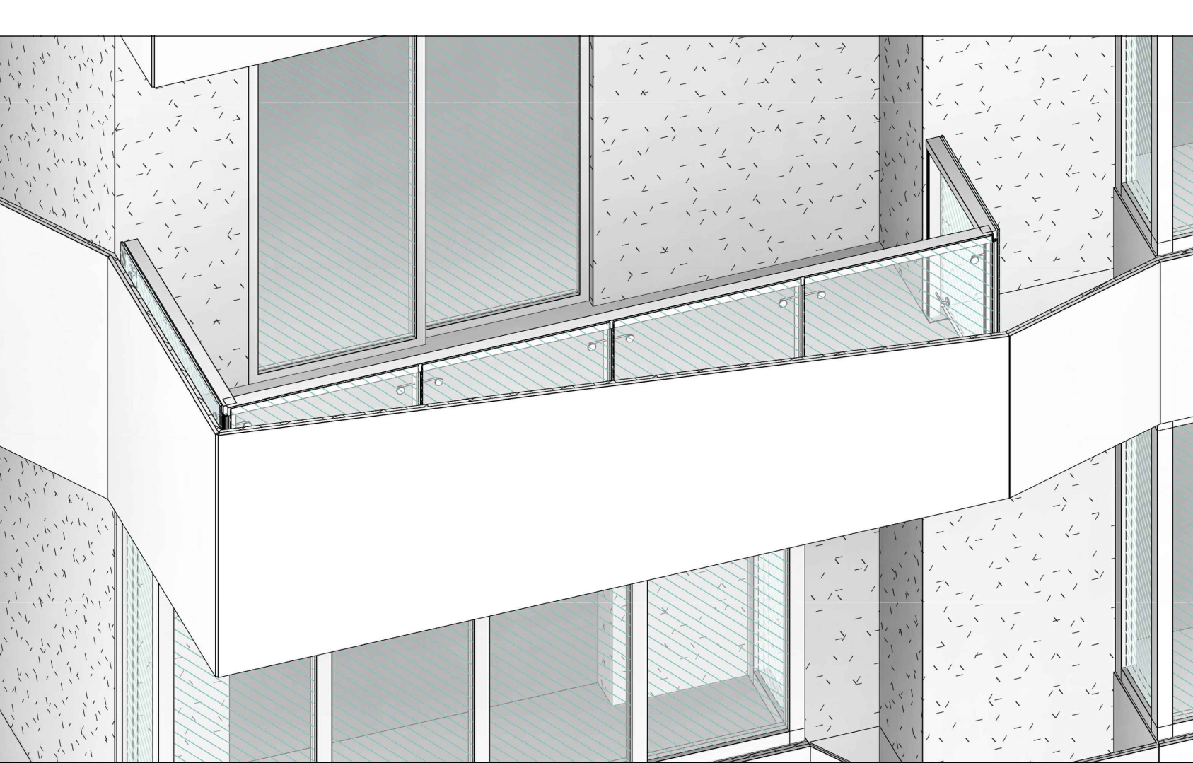
5 3D View Typical balcony SCALE:
