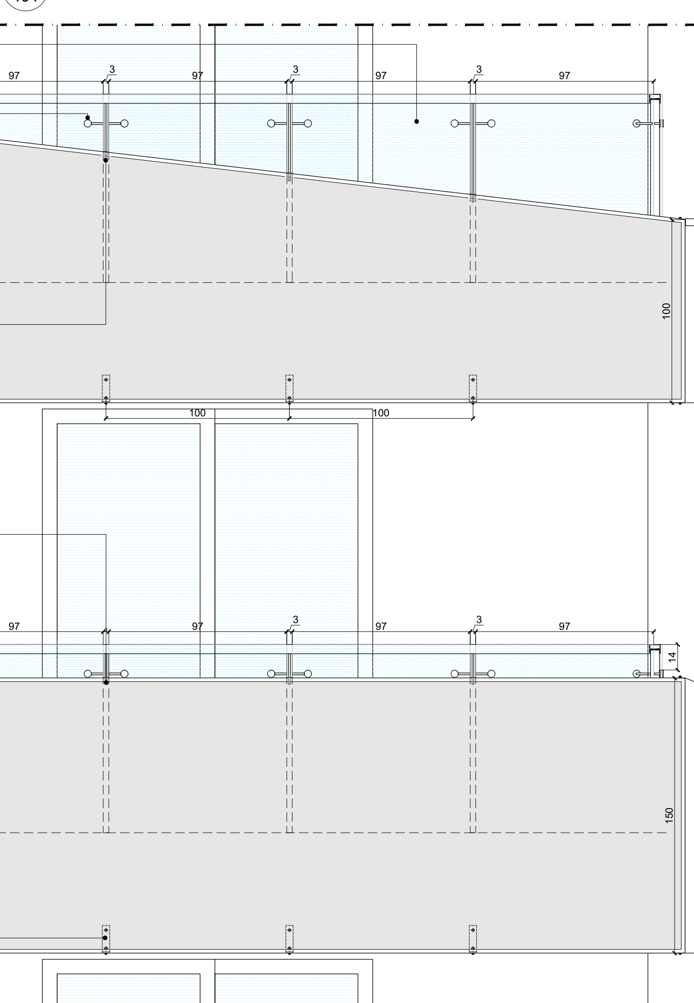
3 Elevation Typical balcony SCALE: 1:20
