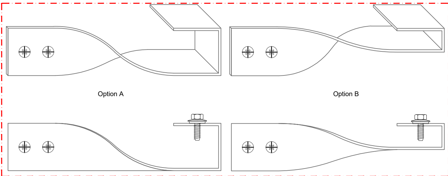
1c Stainless steel flat bars (bent) Examples (to be defined) SCALE: 1:2
