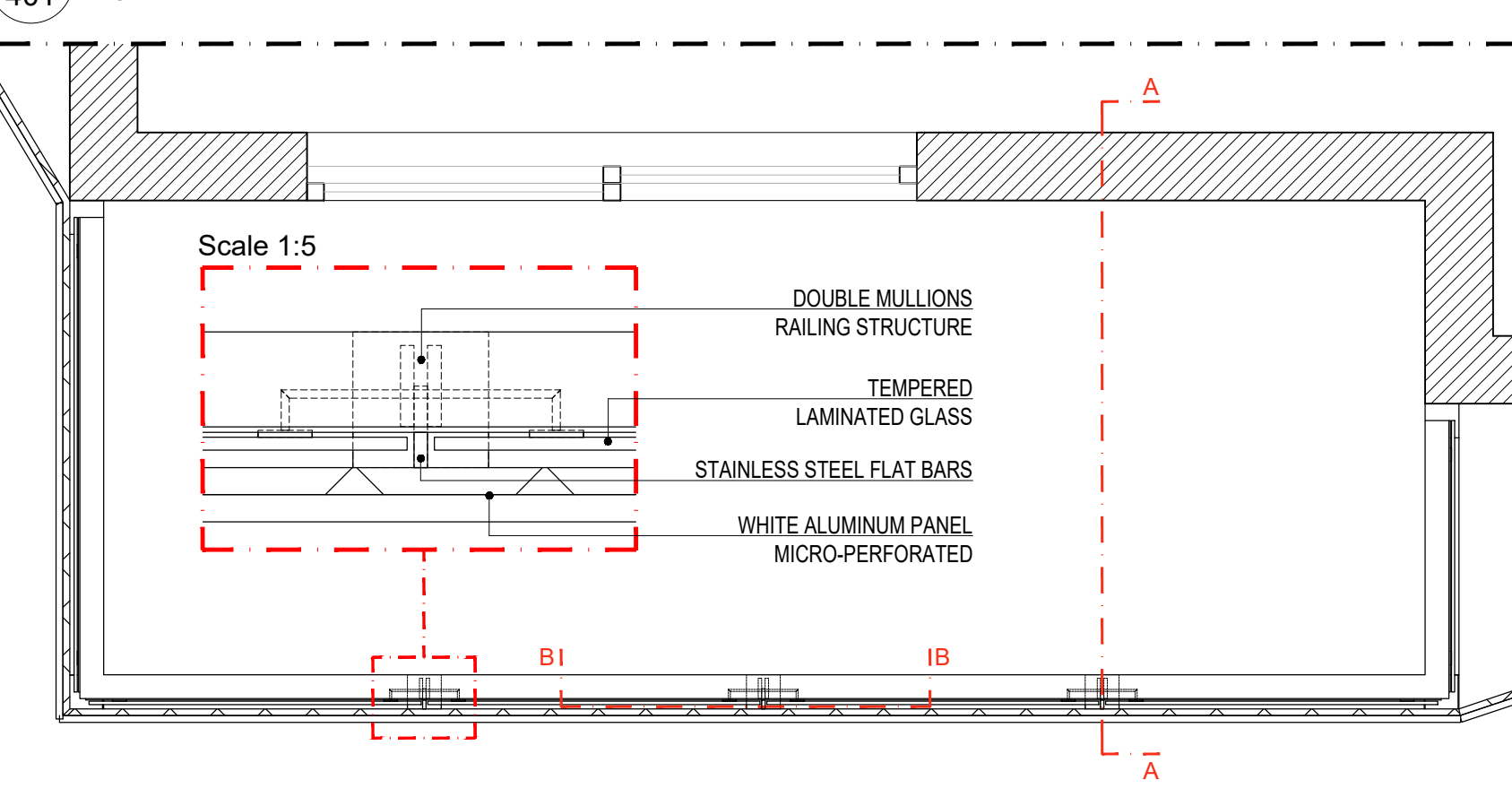
4 Plan Typical balcony SCALE: 1:20
